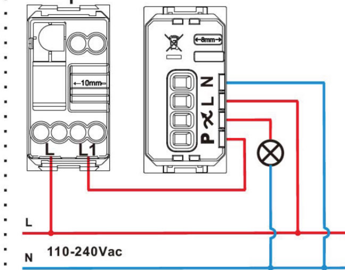
Two-way Switch Mode
