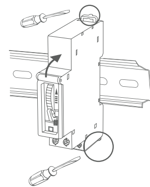
Bottom wiring installation
